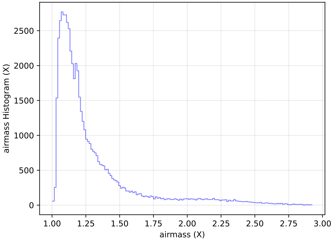
too_elab_r64_d2_griz_v3.4_10yrs Yr 1 i band: airmass Histogram
