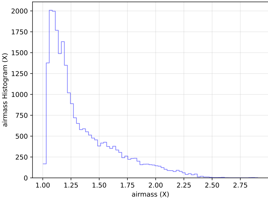
too_elab_r64_d2_griz_v3.4_10yrs Yr 1 g band: airmass Histogram
