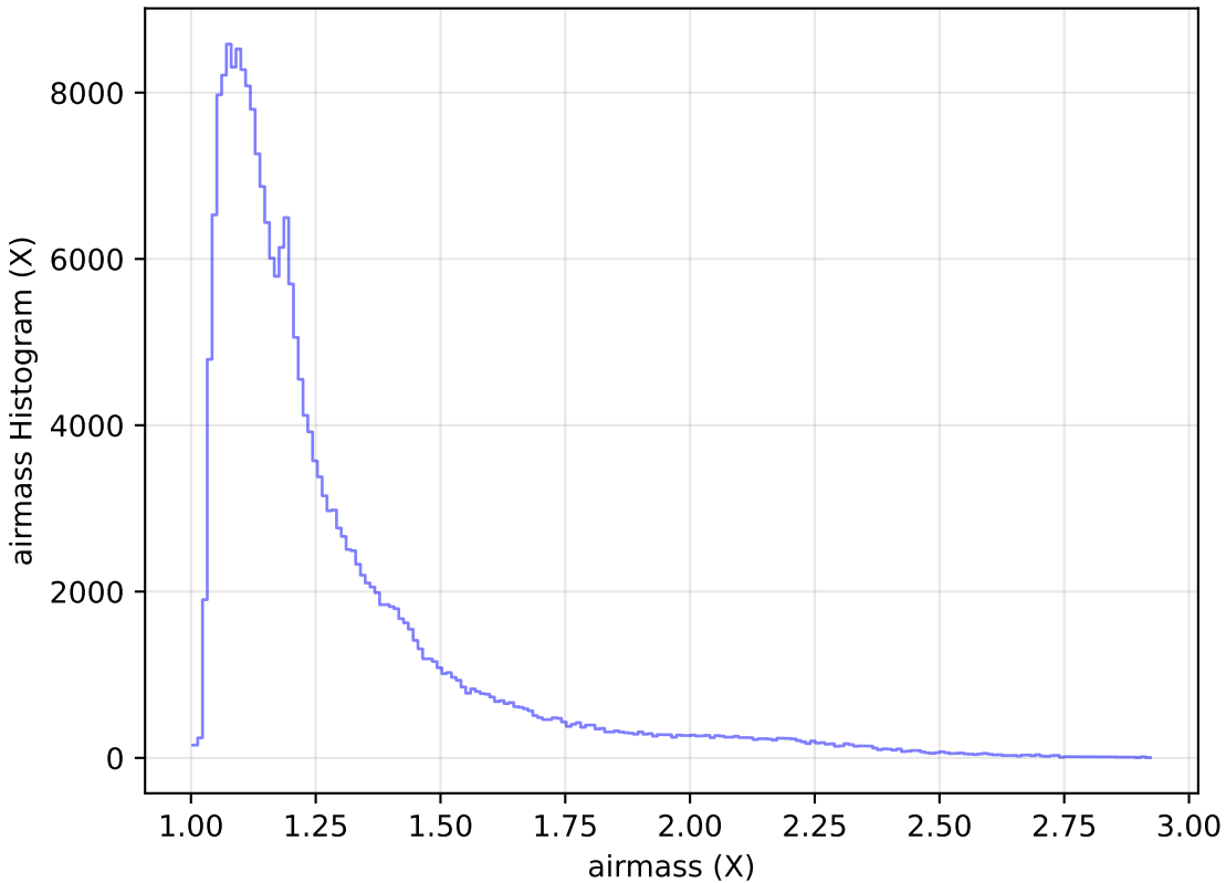
too_elab_r64_d2_griz_v3.4_10yrs Yr 1 all bands: airmass Histogram
