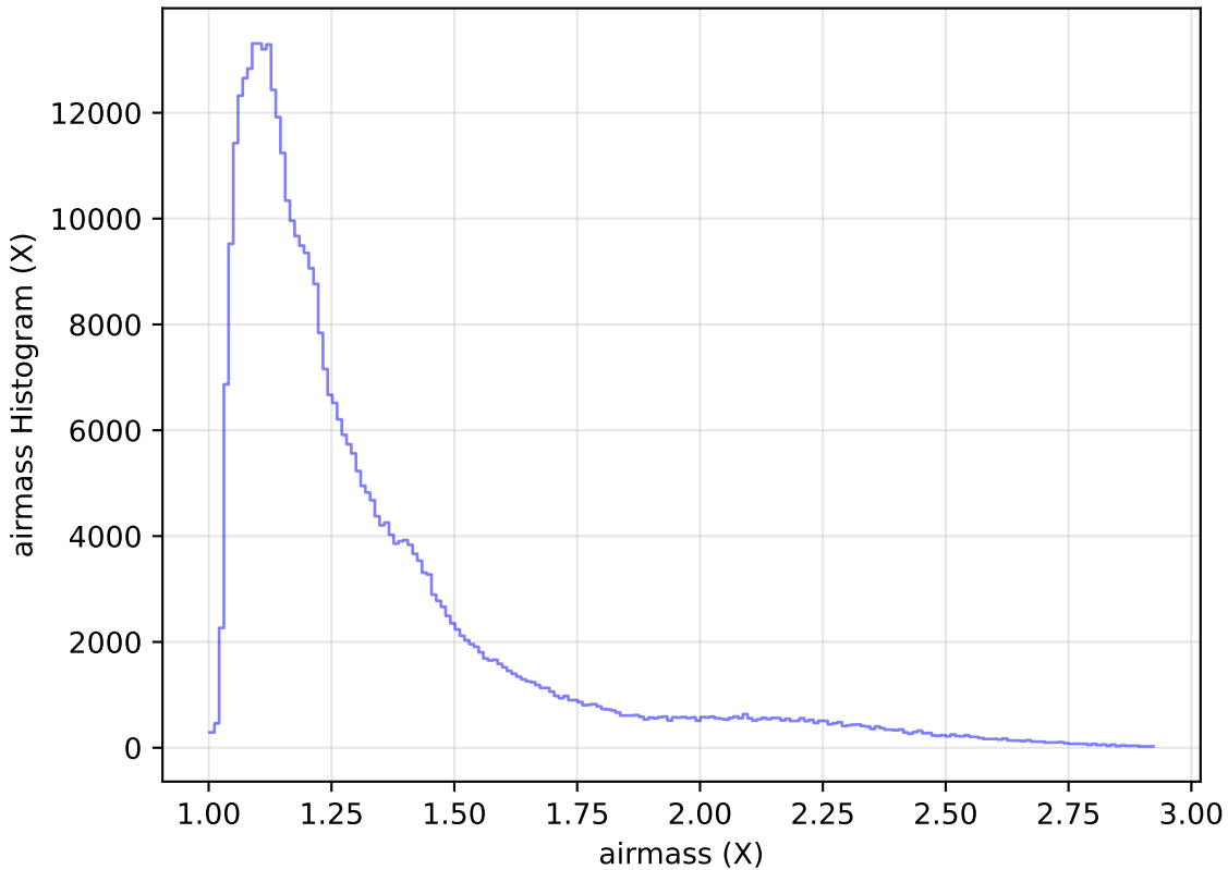
too_elab_r64_d2_griz_v3.4_10yrs WFD z band: airmass Histogram
