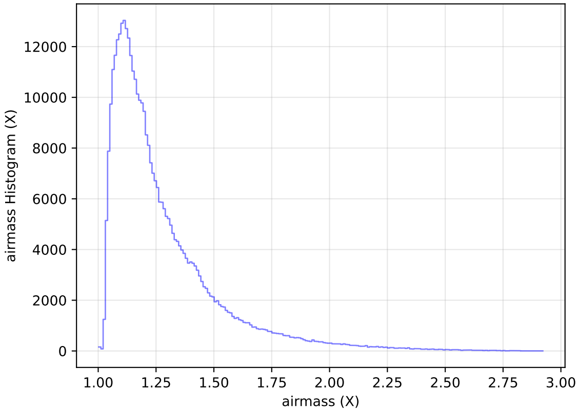
too_elab_r64_d2_griz_v3.4_10yrs WFD y band: airmass Histogram
