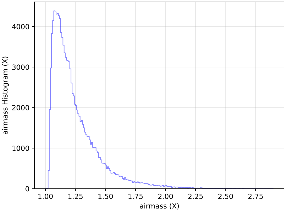
too_elab_r64_d2_griz_v3.4_10yrs WFD u band: airmass Histogram
