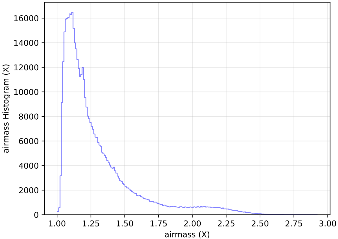
too_elab_r64_d2_griz_v3.4_10yrs WFD r band: airmass Histogram
