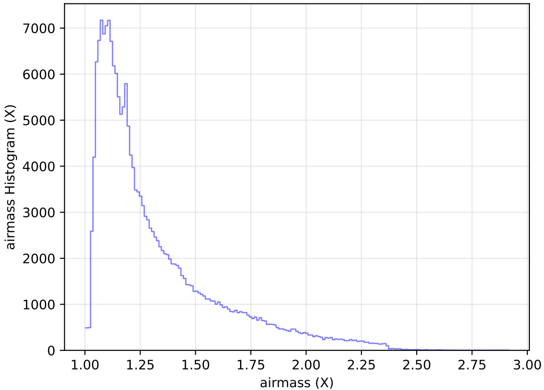
too_elab_r64_d2_griz_v3.4_10yrs WFD g band: airmass Histogram
