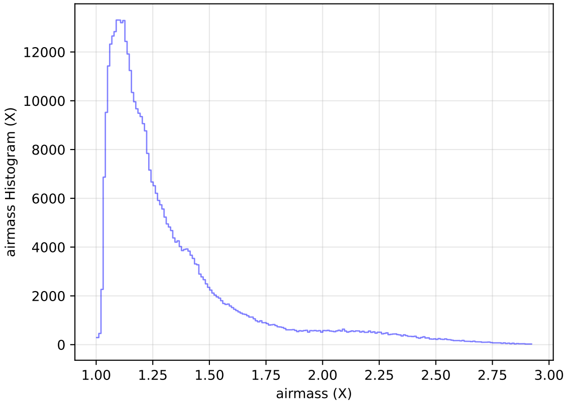
too_elab_r64_d2_griz_v3.4_10yrs All sky z band: airmass Histogram
