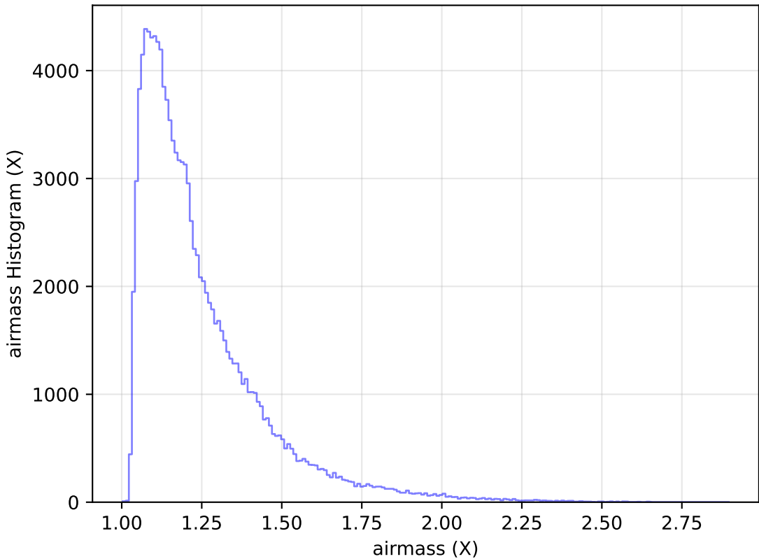
too_elab_r64_d2_griz_v3.4_10yrs All sky u band: airmass Histogram
