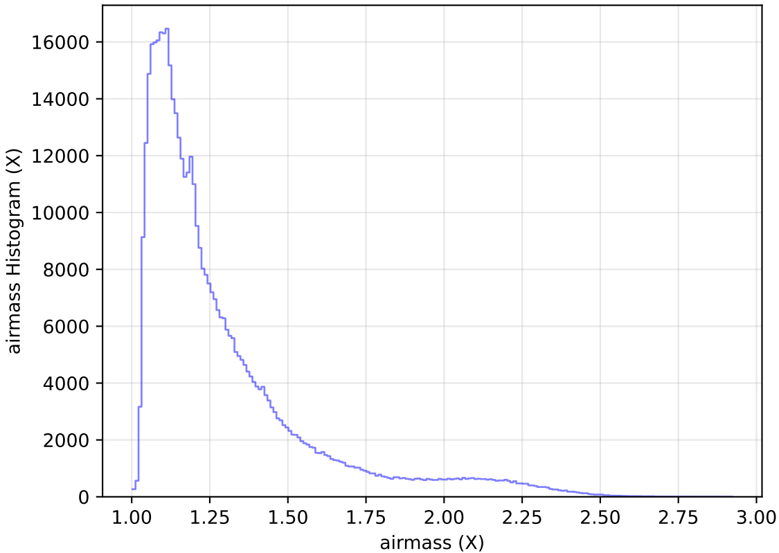
too_elab_r64_d2_griz_v3.4_10yrs All sky r band: airmass Histogram
