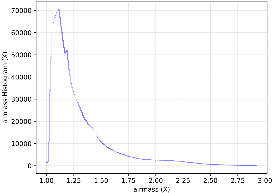
too_elab_r64_d2_griz_v3.4_10yrs All sky all bands: airmass Histogram
