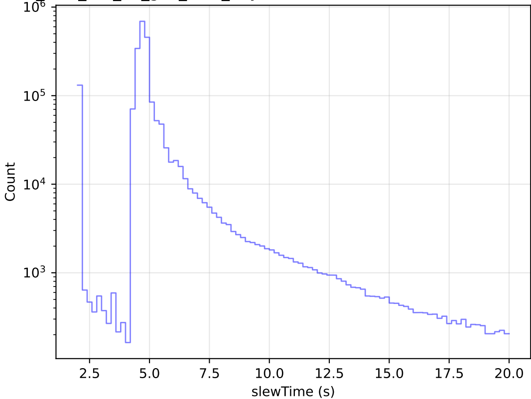
too_elab_r64_d2_griz_v3.4_10yrs All visits: Zoom Slew Time Histogram
