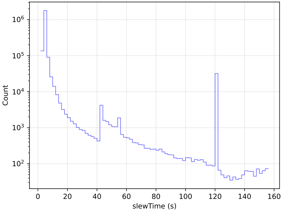
too_elab_r64_d2_griz_v3.4_10yrs All visits: Slew Time Histogram
