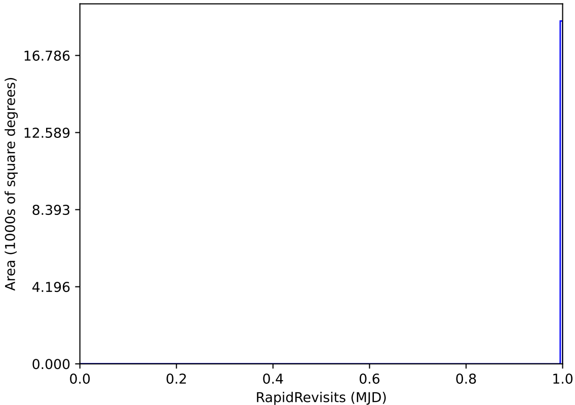
too_elab_r64_d2_griz_v3.4_10yrs WFD: RapidRevisits
