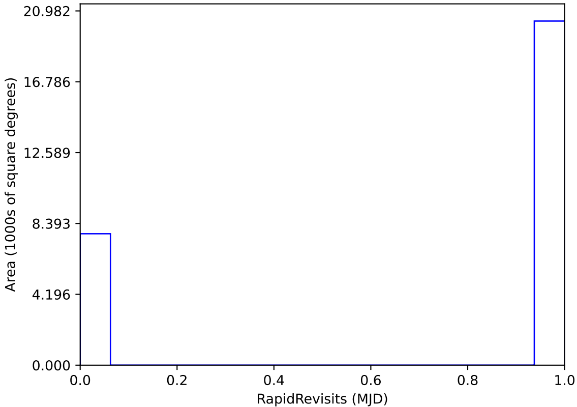
too_elab_r64_d2_griz_v3.4_10yrs All sky: RapidRevisits
