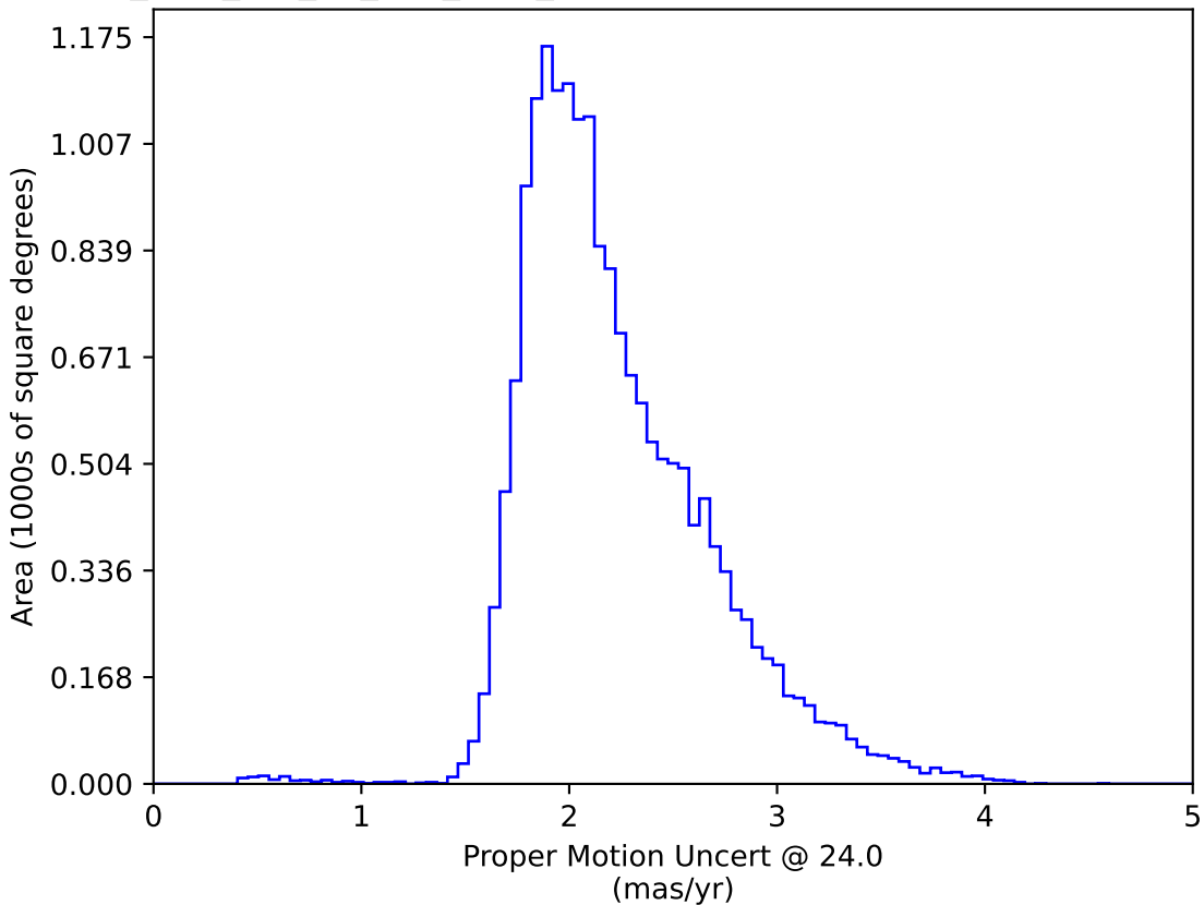
too_elab_r64_d2_griz_v3.4_10yrs WFD: Proper Motion Uncert @ 24.0
