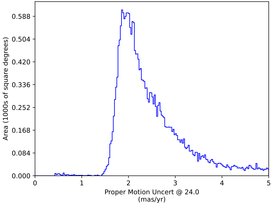
too_elab_r64_d2_griz_v3.4_10yrs All sky: Proper Motion Uncert @ 24.0
