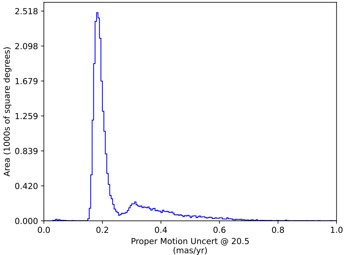
too_elab_r64_d2_griz_v3.4_10yrs All sky: Proper Motion Uncert @ 20.5
