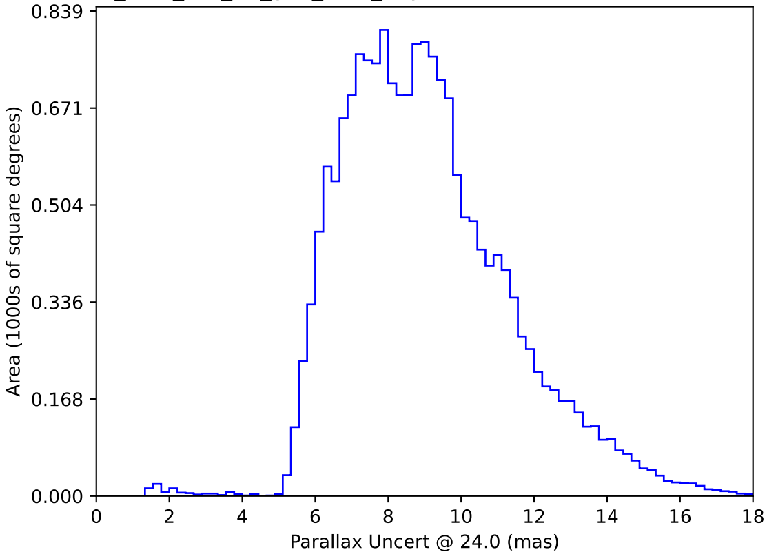
too_elab_r64_d2_griz_v3.4_10yrs WFD: Parallax Uncert @ 24.0
