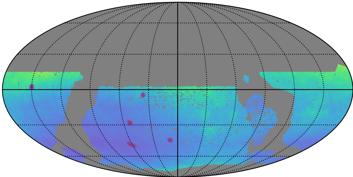
too_elab_r64_d2_griz_v3.4_10yrs WFD: Parallax Uncert @ 22.4
