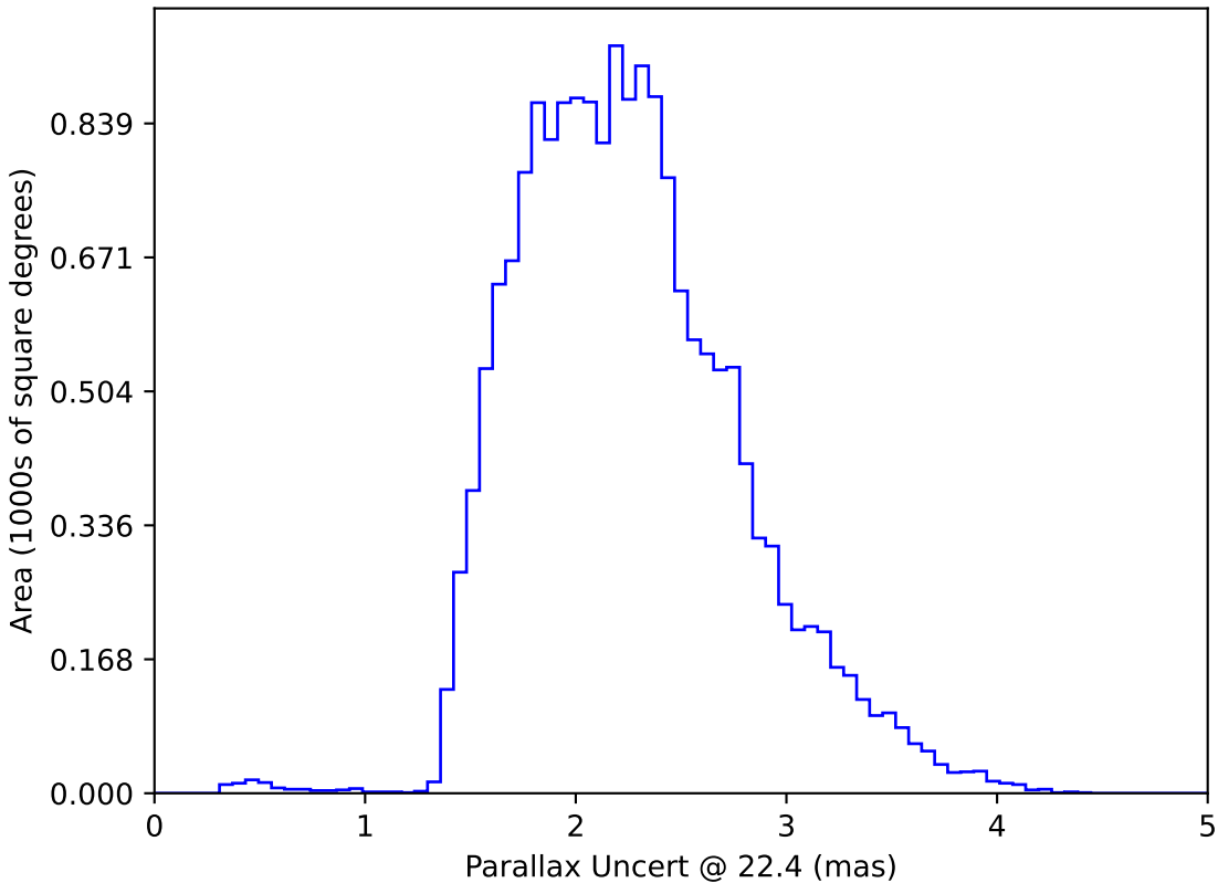
too_elab_r64_d2_griz_v3.4_10yrs WFD: Parallax Uncert @ 22.4
