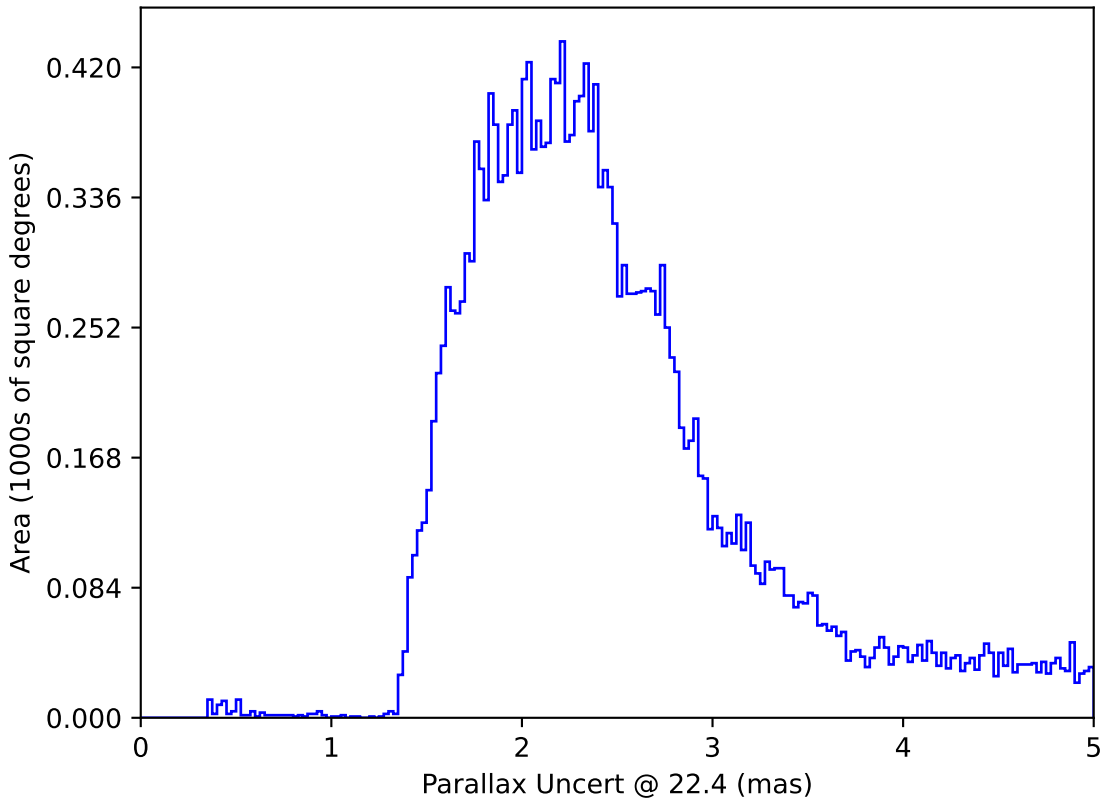
too_elab_r64_d2_griz_v3.4_10yrs All sky: Parallax Uncert @ 22.4
