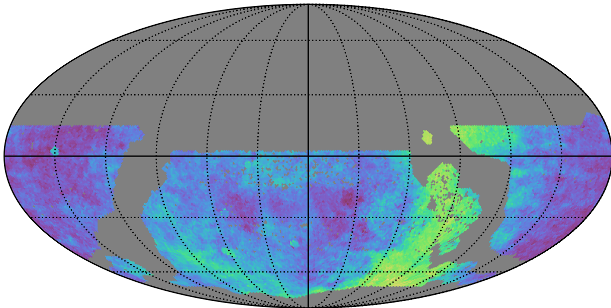
too_elab_r64_d2_griz_v3.4_10yrs WFD: Parallax Coverage @ 24.0
