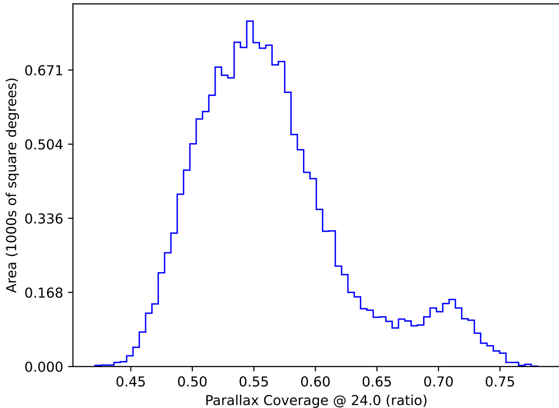
too_elab_r64_d2_griz_v3.4_10yrs WFD: Parallax Coverage @ 24.0
