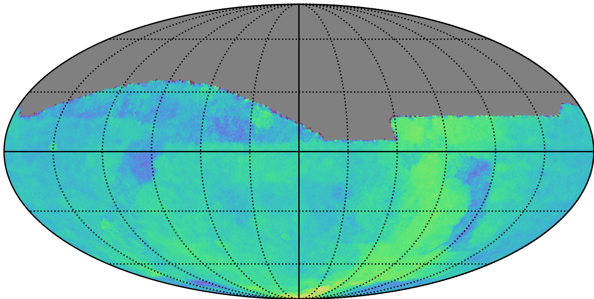
too_elab_r64_d2_griz_v3.4_10yrs All sky: Parallax Coverage @ 24.0
