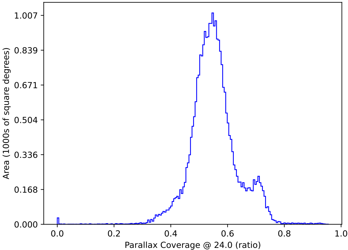
too_elab_r64_d2_griz_v3.4_10yrs All sky: Parallax Coverage @ 24.0
