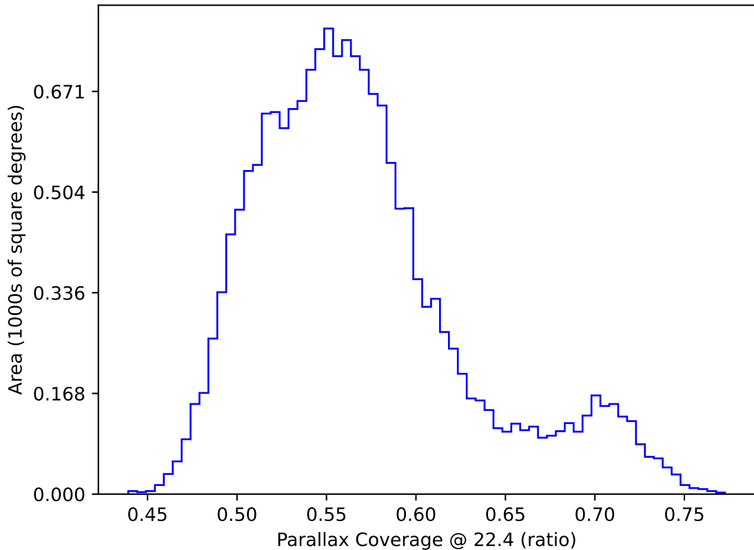
too_elab_r64_d2_griz_v3.4_10yrs WFD: Parallax Coverage @ 22.4
