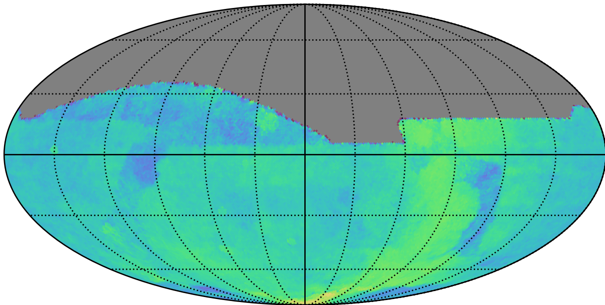
too_elab_r64_d2_griz_v3.4_10yrs All sky: Parallax Coverage @ 22.4
