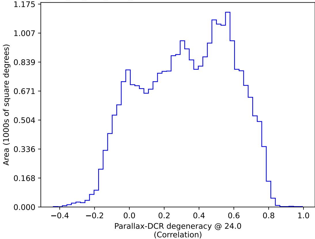
too_elab_r64_d2_griz_v3.4_10yrs All sky: Parallax-DCR degeneracy @ 24.0
