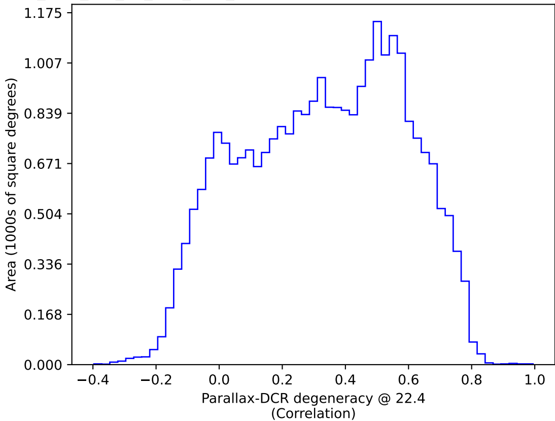
too_elab_r64_d2_griz_v3.4_10yrs All sky: Parallax-DCR degeneracy @ 22.4
