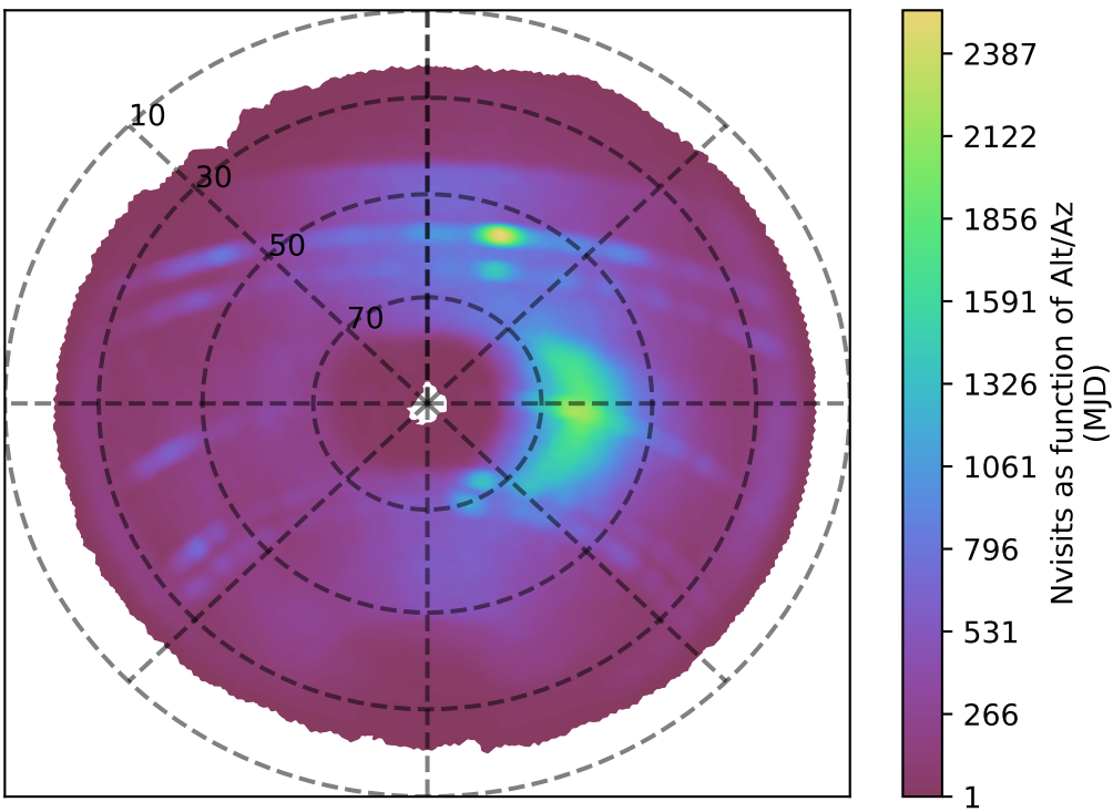
too_elab_r64_d2_griz_v3.4_10yrs z band: Nvisits as function of Alt/Az
