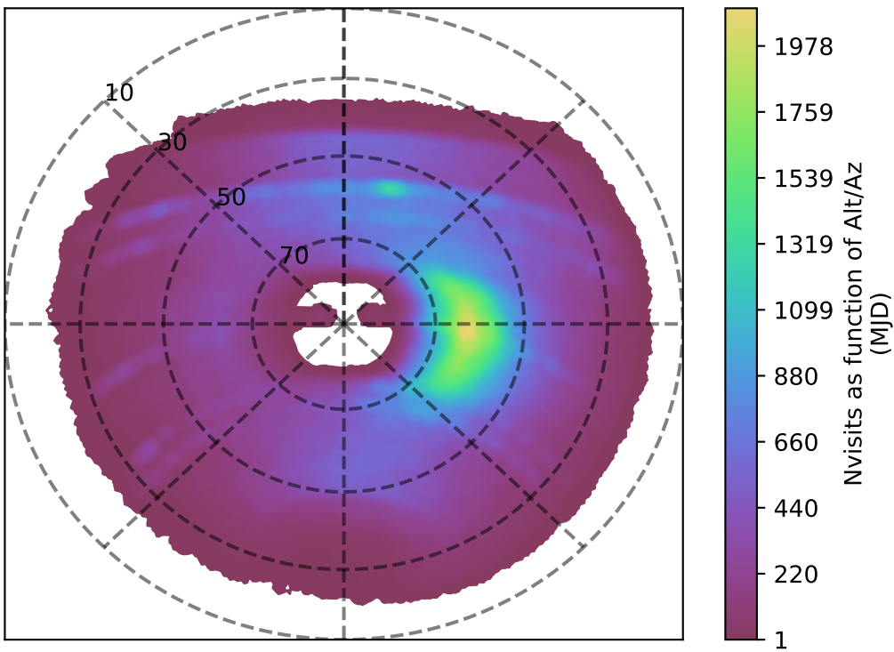
too_elab_r64_d2_griz_v3.4_10yrs y band: Nvisits as function of Alt/Az
