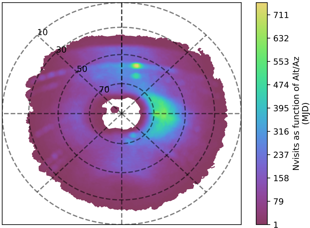
too_elab_r64_d2_griz_v3.4_10yrs u band: Nvisits as function of Alt/Az
