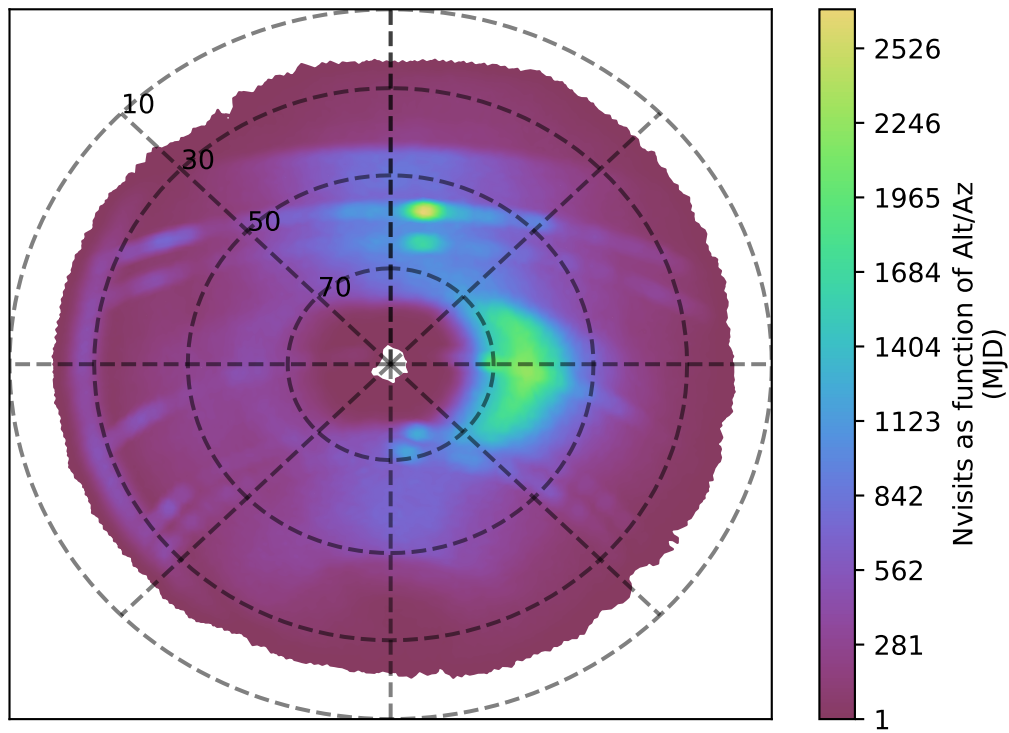
too_elab_r64_d2_griz_v3.4_10yrs r band: Nvisits as function of Alt/Az
