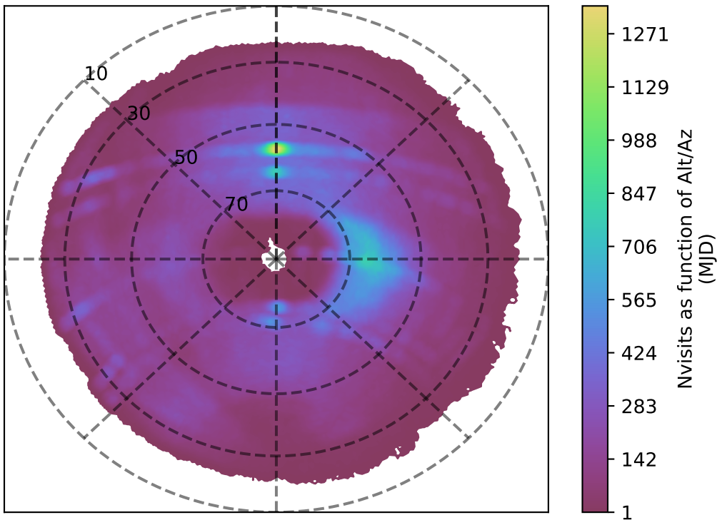
too_elab_r64_d2_griz_v3.4_10yrs g band: Nvisits as function of Alt/Az
