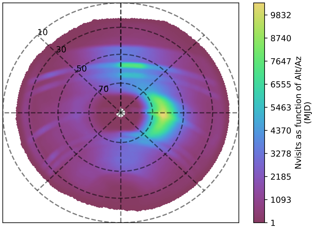
too_elab_r64_d2_griz_v3.4_10yrs all bands: Nvisits as function of Alt/Az
