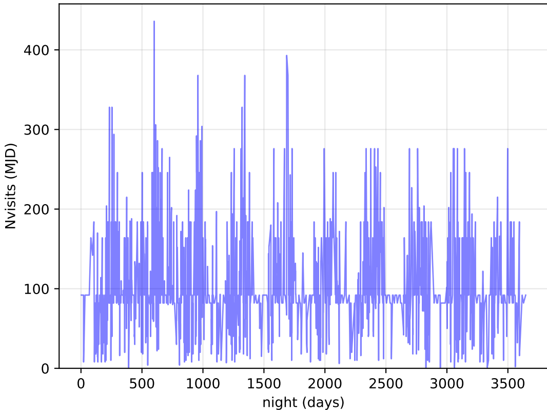
too_elab_r64_d2_griz_v3.4_10yrs DDF: Nvisits
