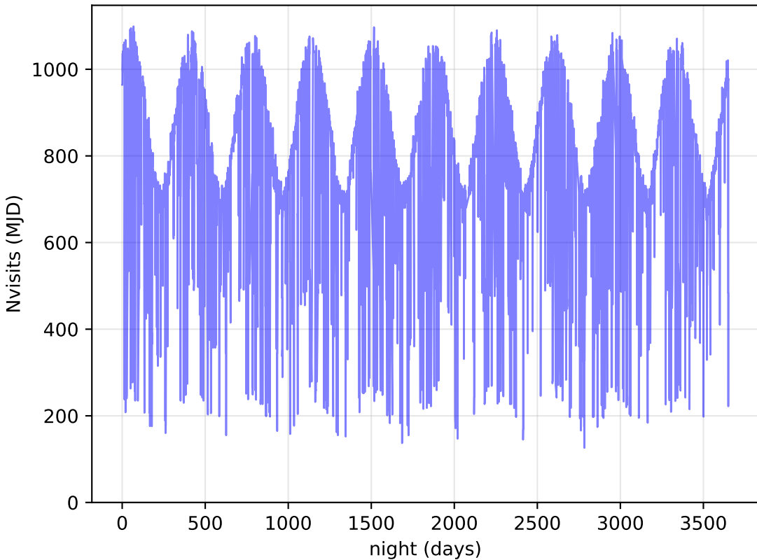
too_elab_r64_d2_griz_v3.4_10yrs All visits: Nvisits
