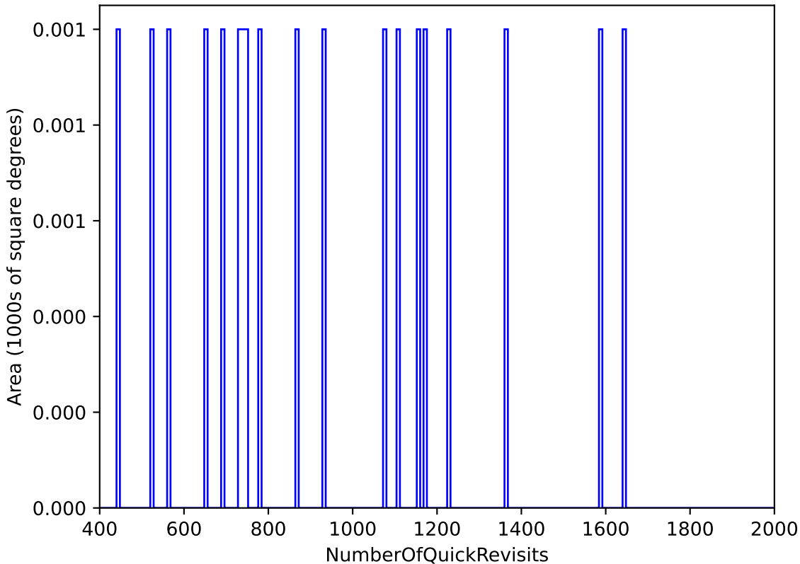
too_elab_r64_d2_griz_v3.4_10yrs WFD: NumberOfQuickRevisits
