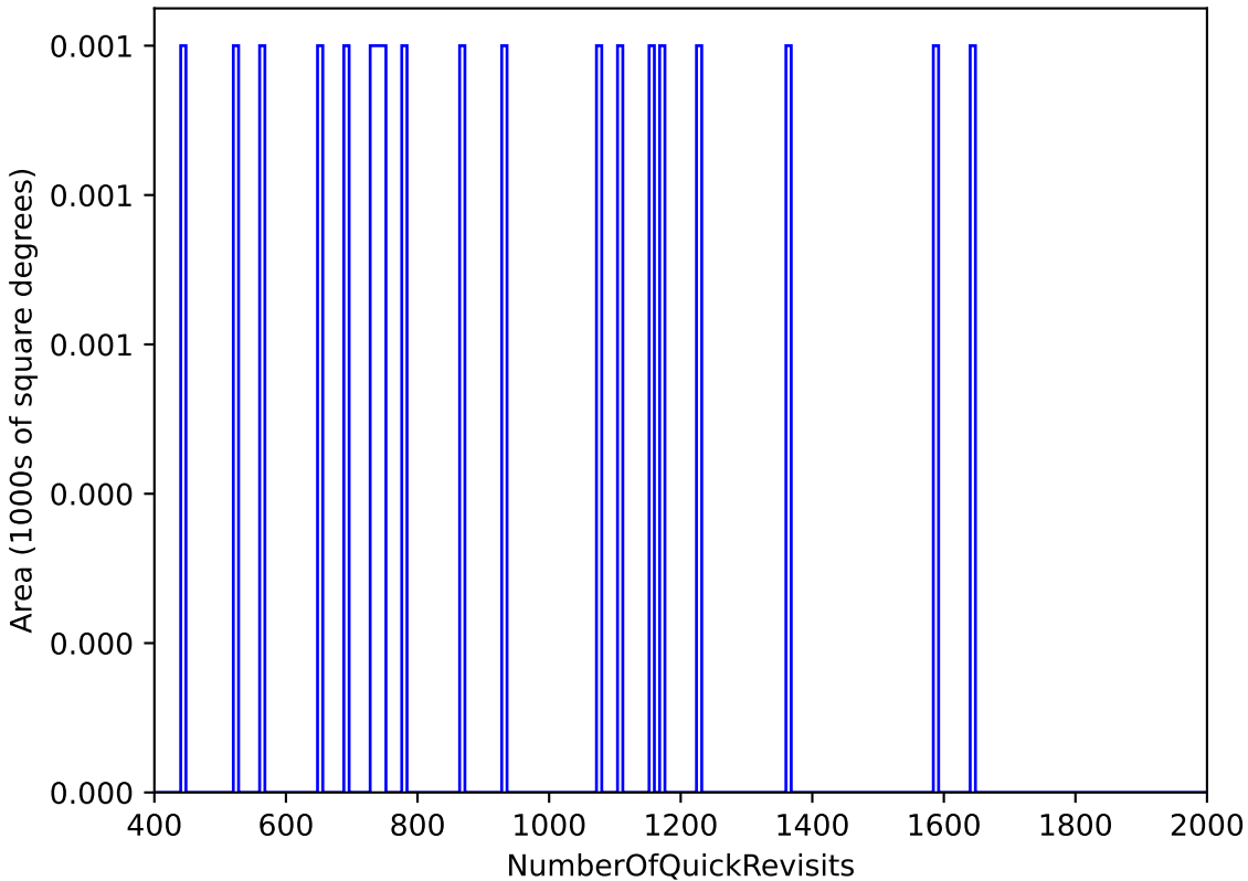
too_elab_r64_d2_griz_v3.4_10yrs All sky: NumberOfQuickRevisits
