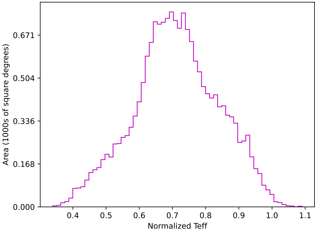
too_elab_r64_d2_griz_v3.4_10yrs WFD z band: Normalized Teff
