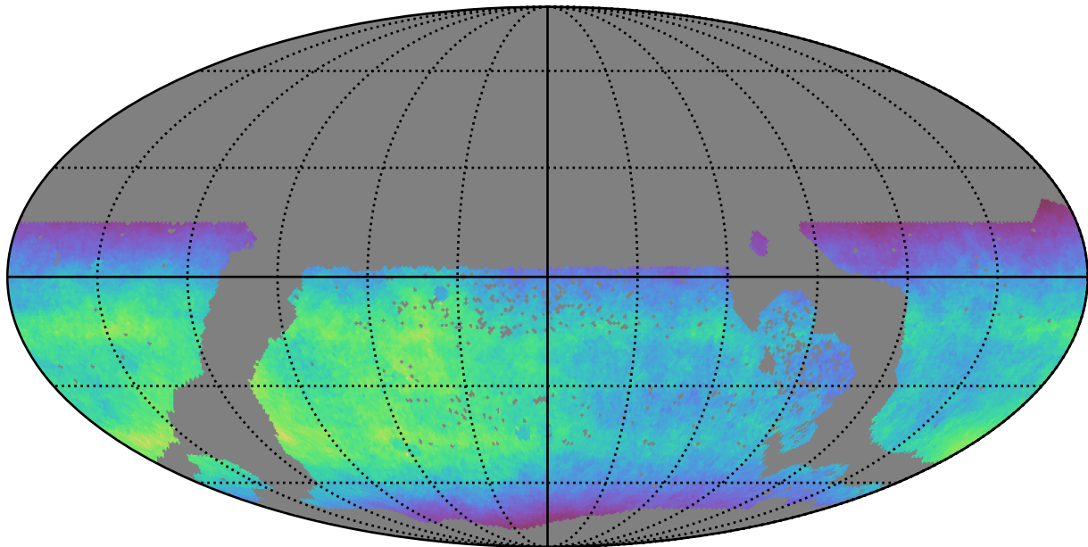
too_elab_r64_d2_griz_v3.4_10yrs WFD y band: Normalized Teff
