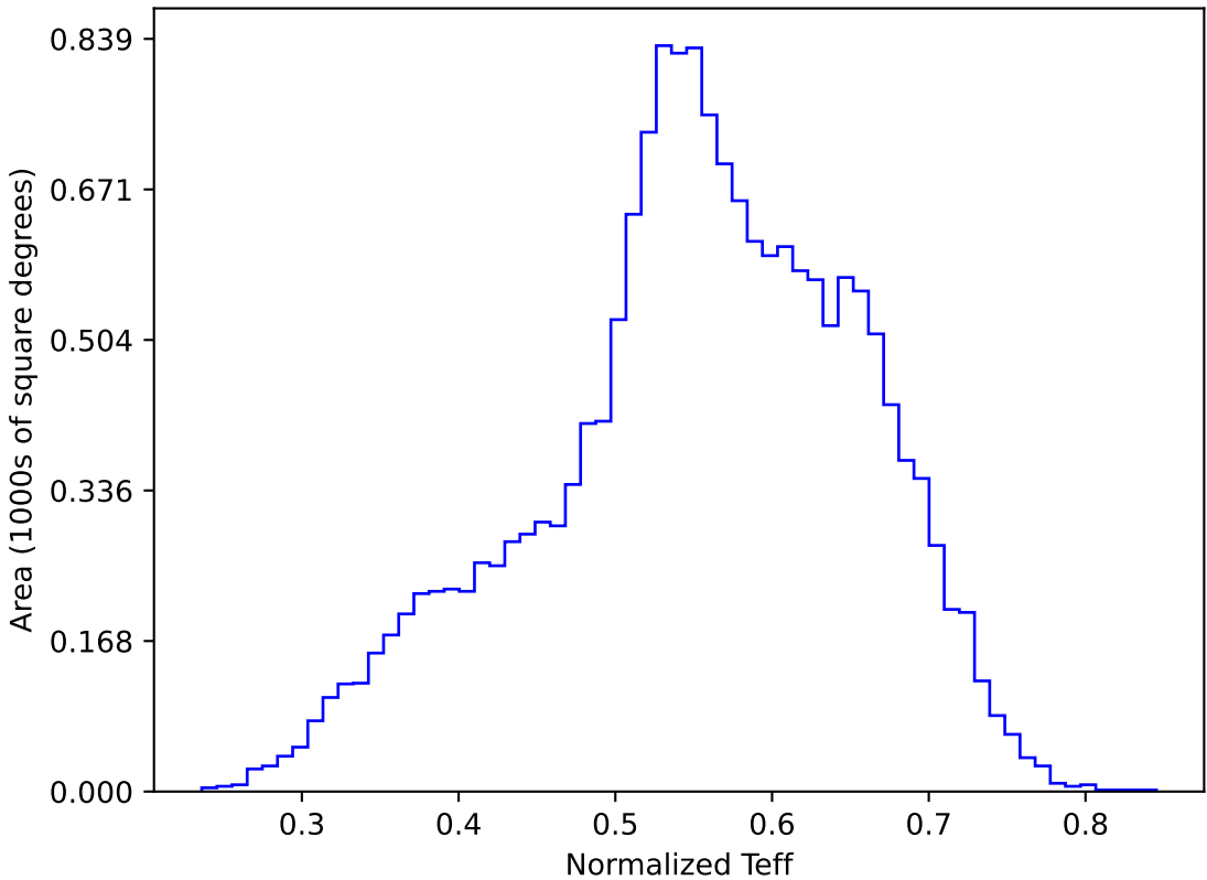
too_elab_r64_d2_griz_v3.4_10yrs WFD y band: Normalized Teff
