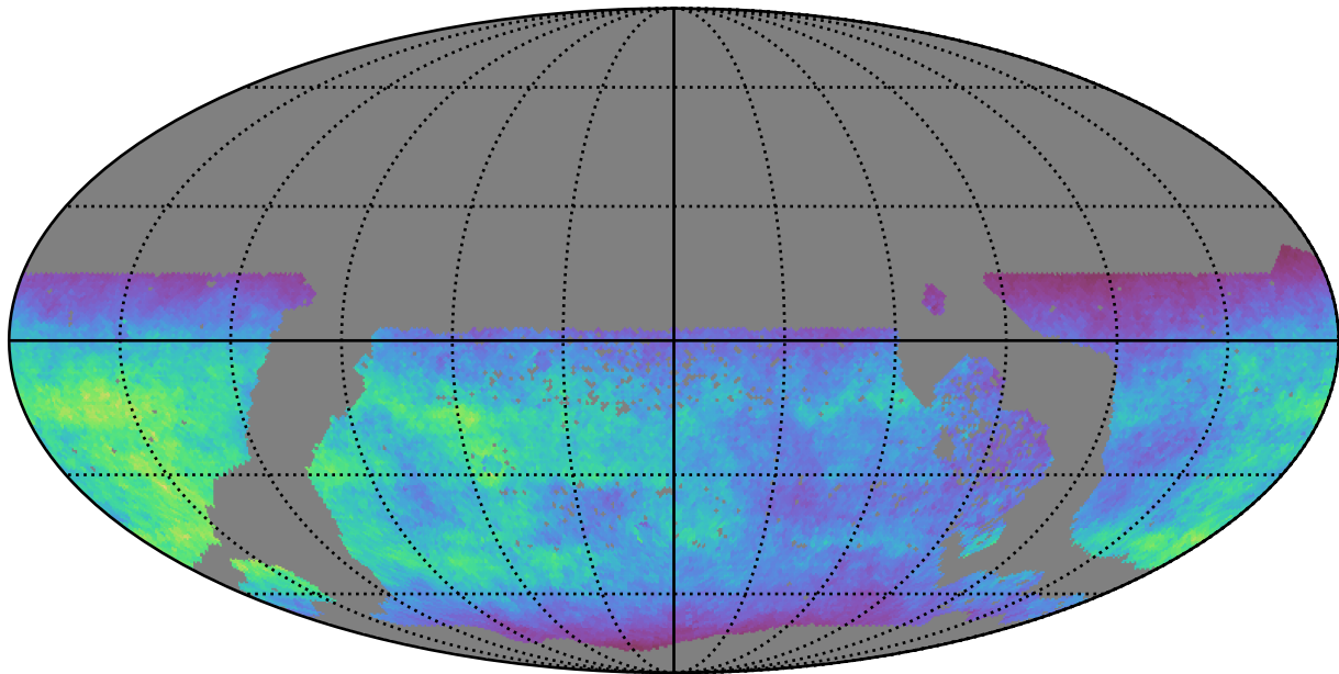
too_elab_r64_d2_griz_v3.4_10yrs WFD u band: Normalized Teff
