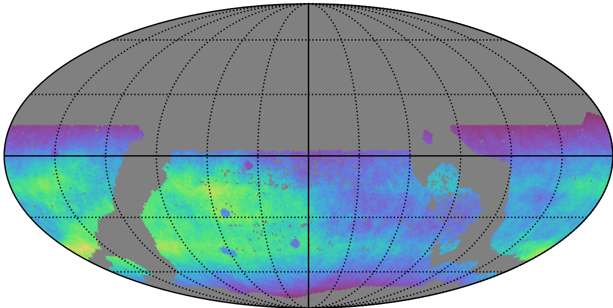
too_elab_r64_d2_griz_v3.4_10yrs WFD r band: Normalized Teff
