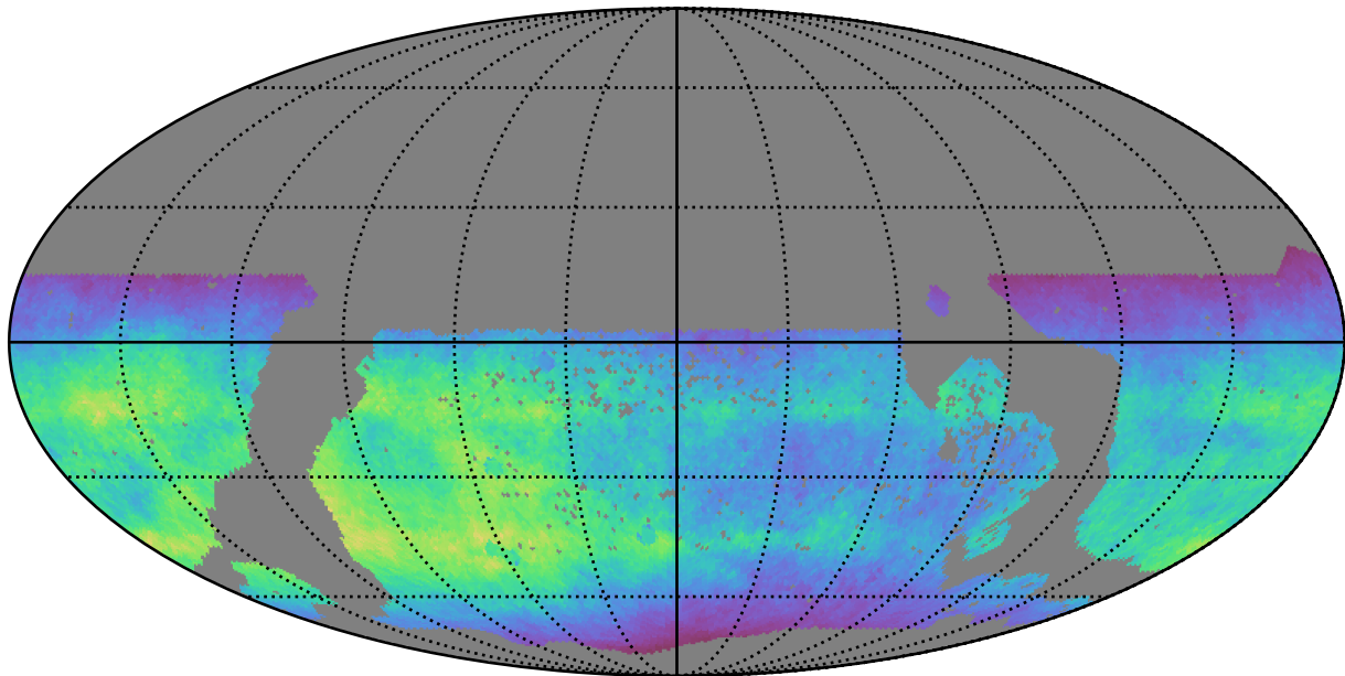
too_elab_r64_d2_griz_v3.4_10yrs WFD i band: Normalized Teff
