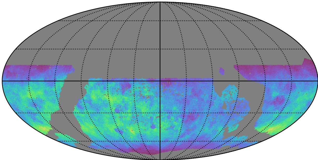
too_elab_r64_d2_griz_v3.4_10yrs WFD g band: Normalized Teff
