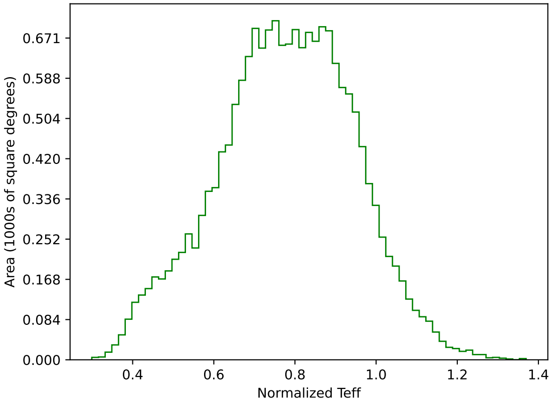
too_elab_r64_d2_griz_v3.4_10yrs WFD g band: Normalized Teff
