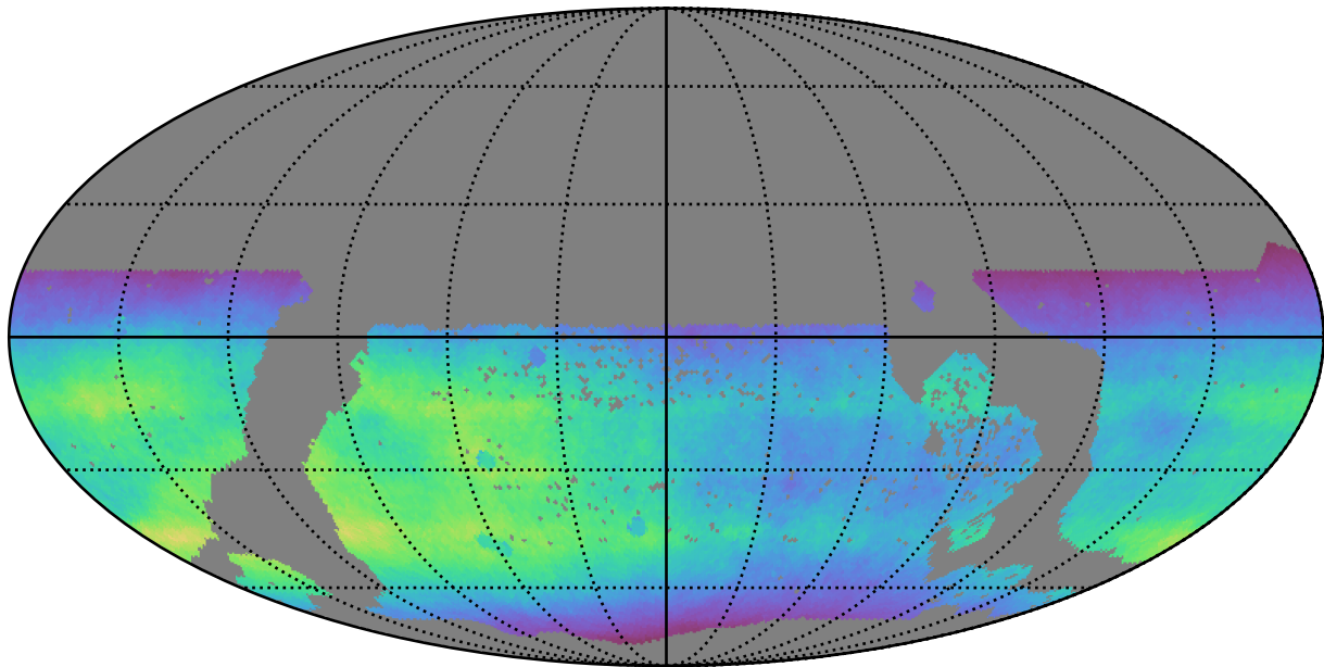
too_elab_r64_d2_griz_v3.4_10yrs WFD all bands: Normalized Teff
